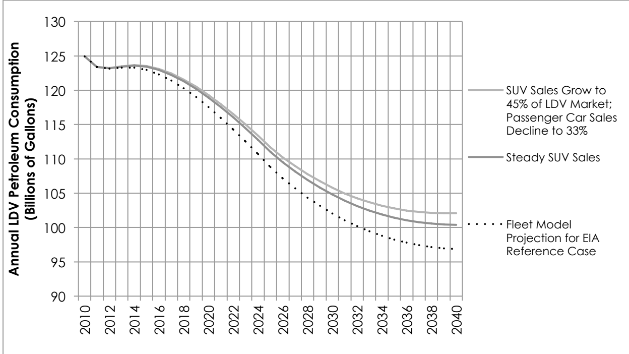
Figure 34: Annual LDV fuel consumption projections for strong SUV sales scenarios, 2010 through 2040
