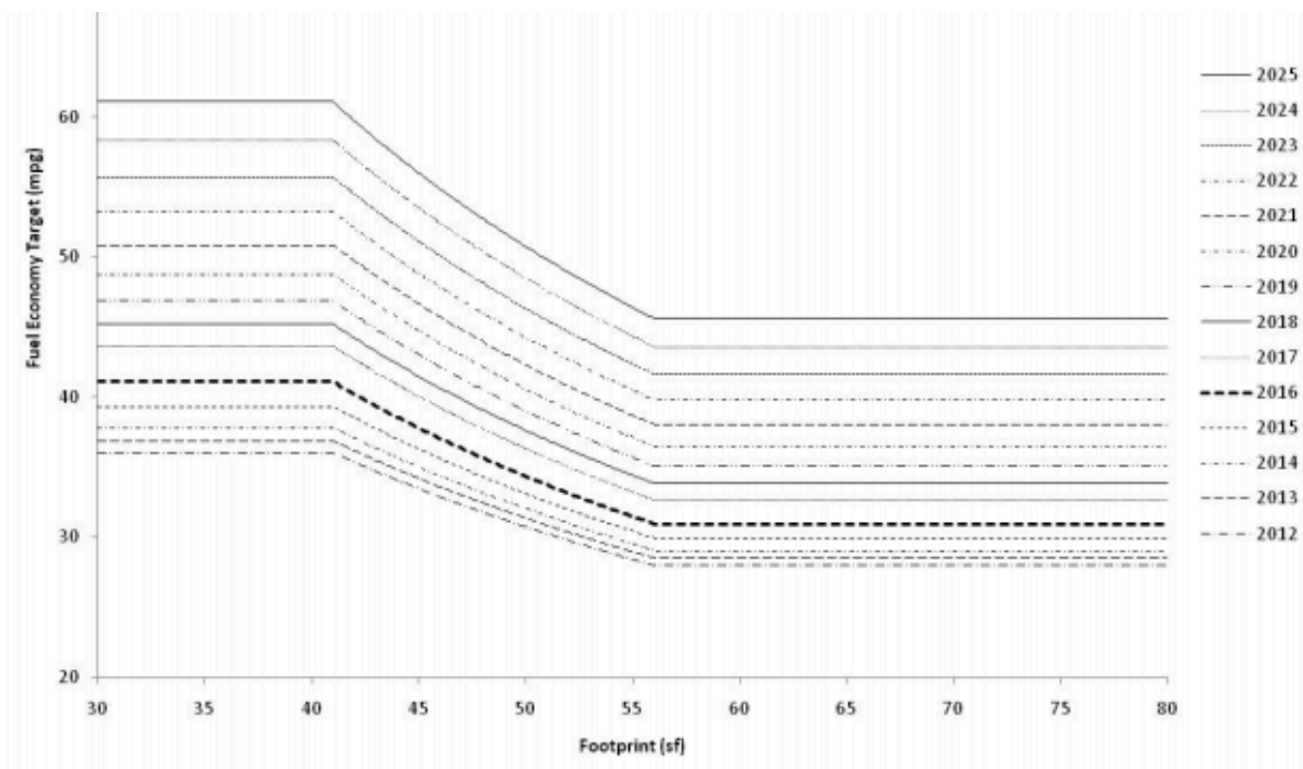
Figure 36: Footprint-based passenger car CAFE targets for model years 2012 through 2025 (Source: NHTSA)
